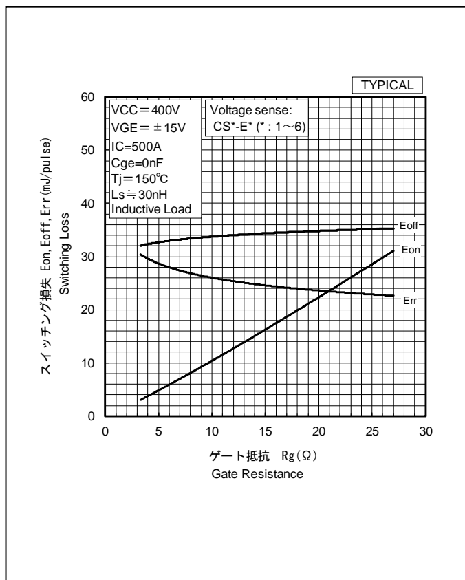
Switching Loss vs. Gate Resistance
