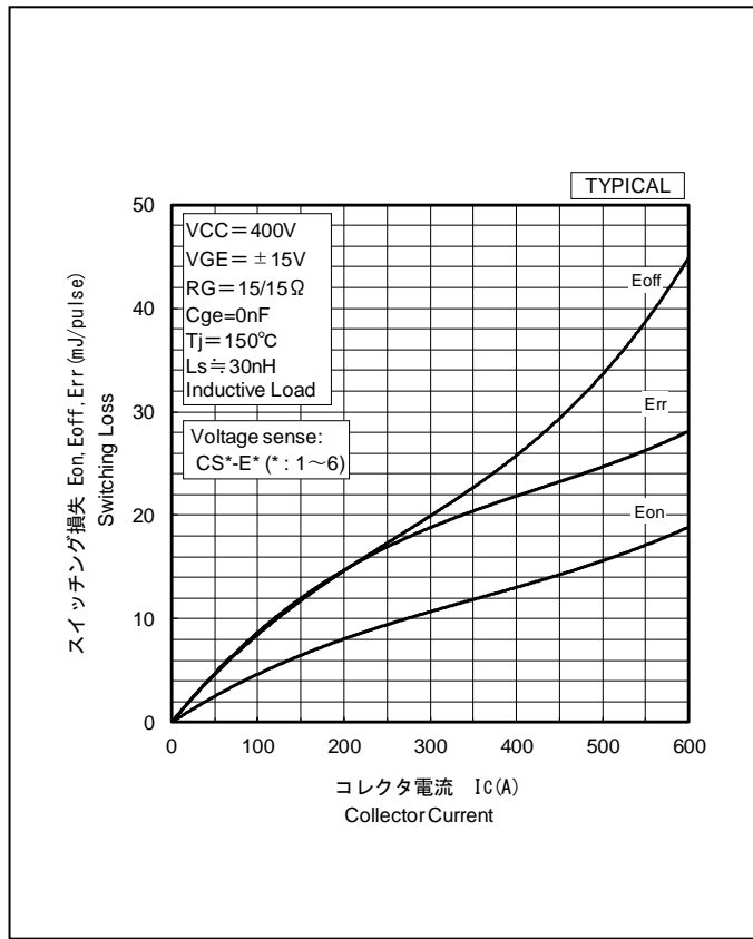
Switching Loss vs. Collector Current
