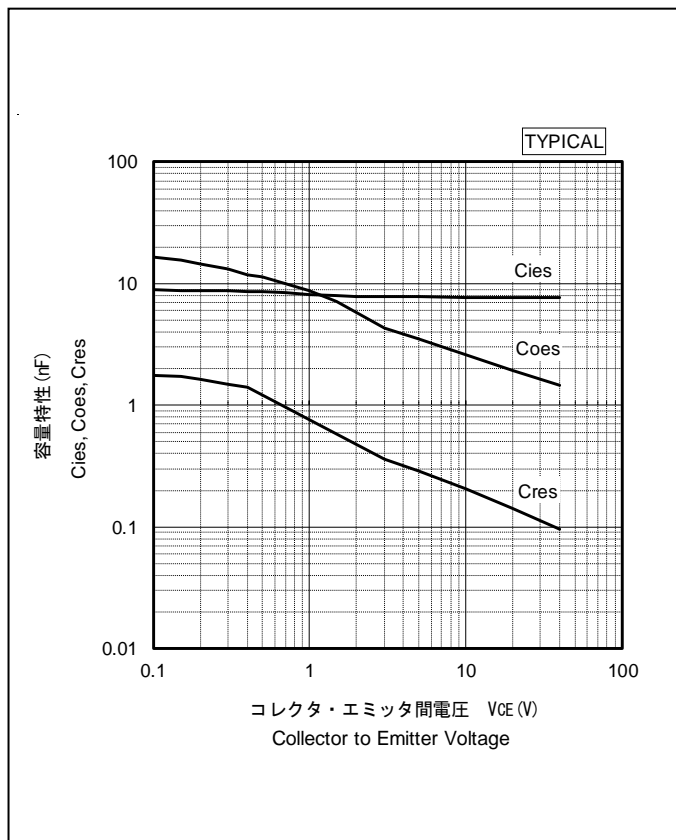
Capacitance Characteristics
