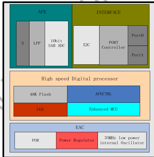
Figure 2-1 FT6336U System Architecture Diagram
